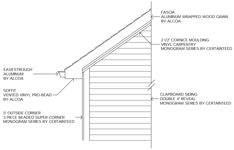
"BOX" RETURN
