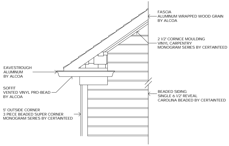
"SHINGLE" RETURN
