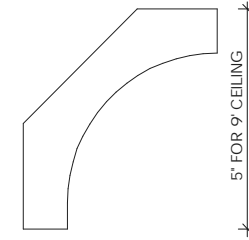
CROWN MOULDING - COVE PROFILE
