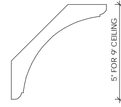
CROWN MOULDING - OPTIONAL BEADED PROFILE
