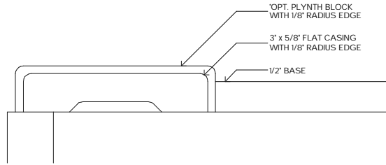
CASING PROFILES - TOP VIEW
