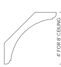
CROWN MOULDING - OPTIONAL BEADED PROFILE
