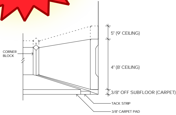
BASEBOARD
