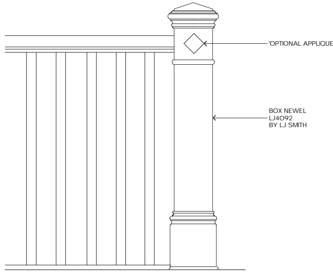
STAIR DETAIL
