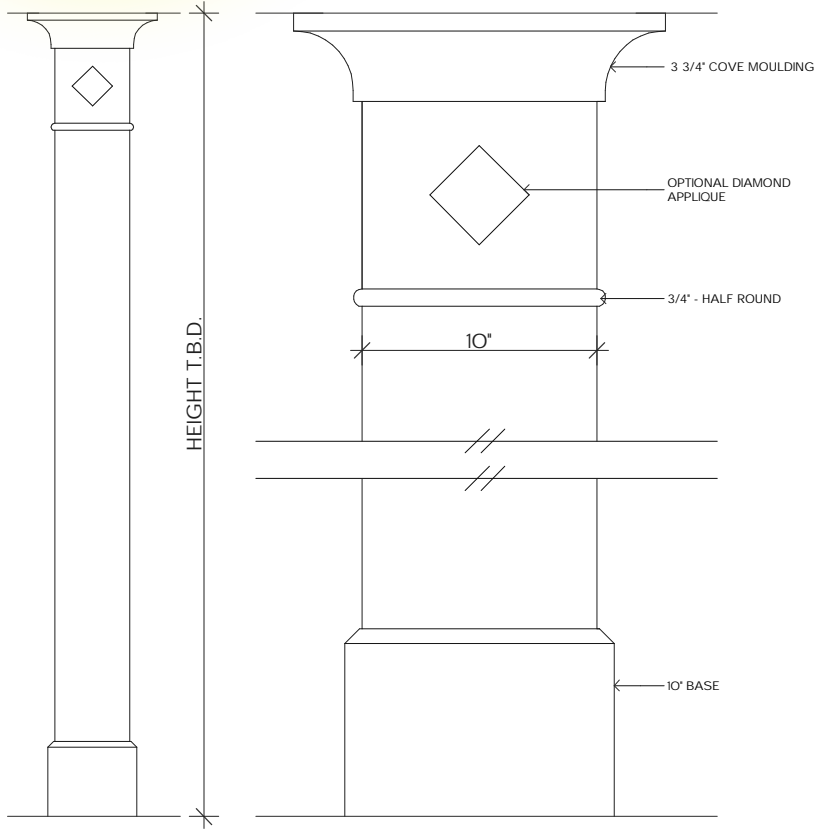
COLUMN DETAIL
