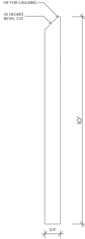
BASE MOULDING
