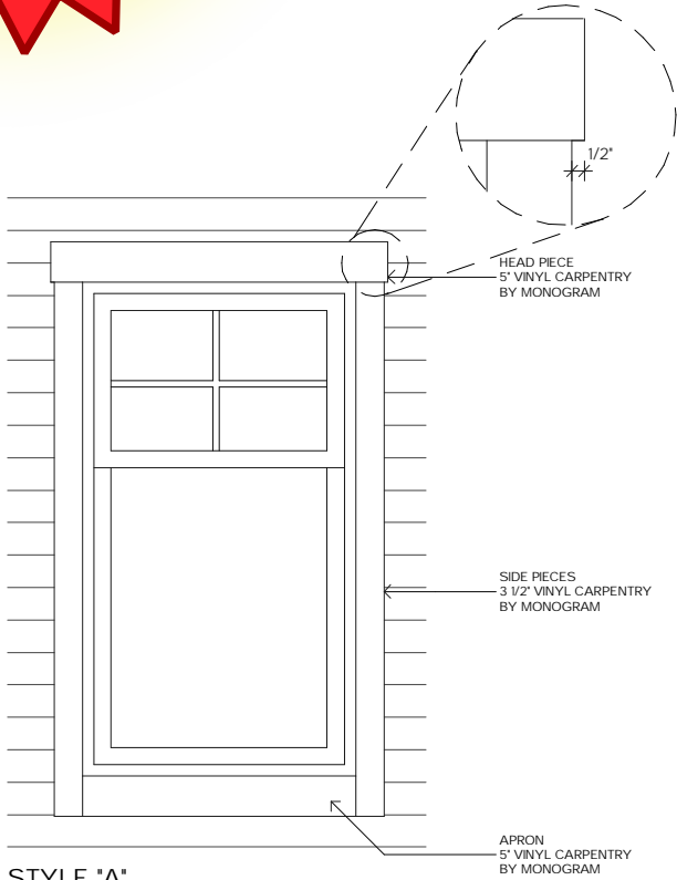
STYLE "A" CROSSBAR MUNTIN PATTERN
