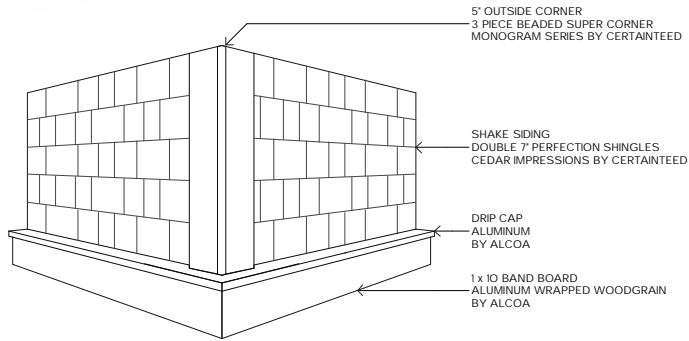
OUTSIDE CORNER DETAIL
